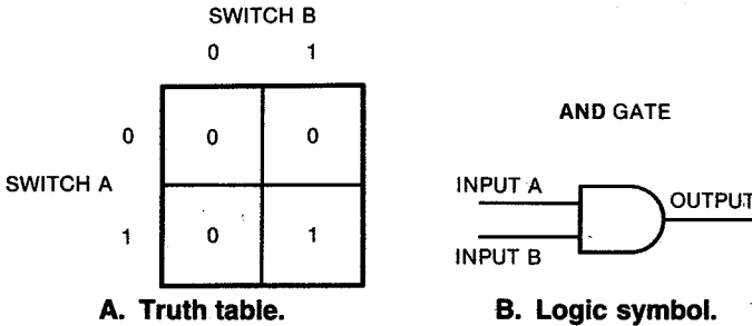
Fig. 1-10. An AND gate.
